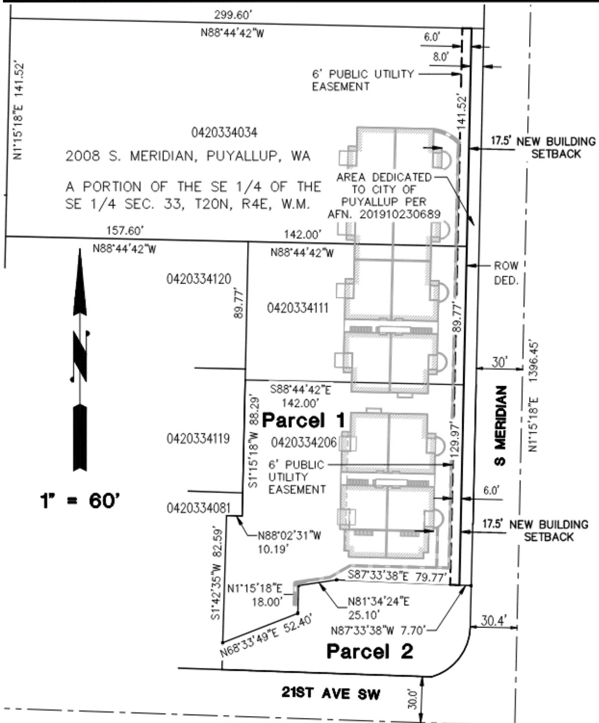
Site Plan
