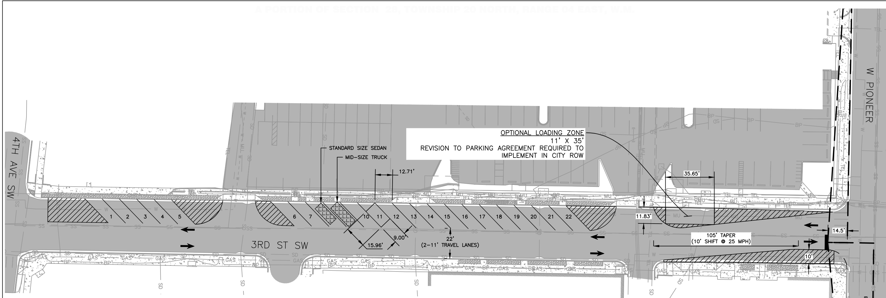
3RD ST SW PROPOSED CONDITIONS SCALE: 1" = 40' (TWO WAY TRAFFIC WITH 45° ANGLED STREET PARKING SOUTHBOUND ONLY)
